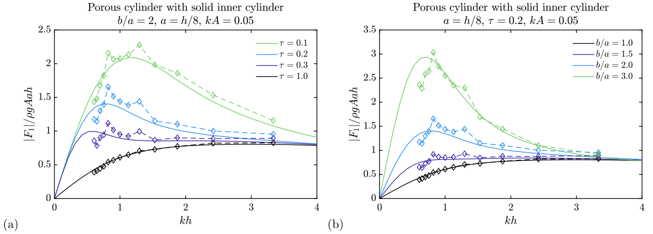
Fig. 9. Nondimensional amplitude of horizontal force on fixed porous cylinder with solid inner cylinder from BEM model (solid line) and measurements (diamonds). (a) For outer cylinders of various porosities. (b) For outer cylinders of various radii.
