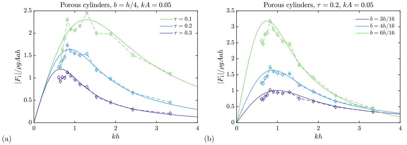
Fig. 7. Nondimensional amplitude of horizontal force on fixed porous cylinder from BEM model (solid line) and measurements (diamonds). (a) For various cylinder porosities. (b) For cylinders of various radii.
