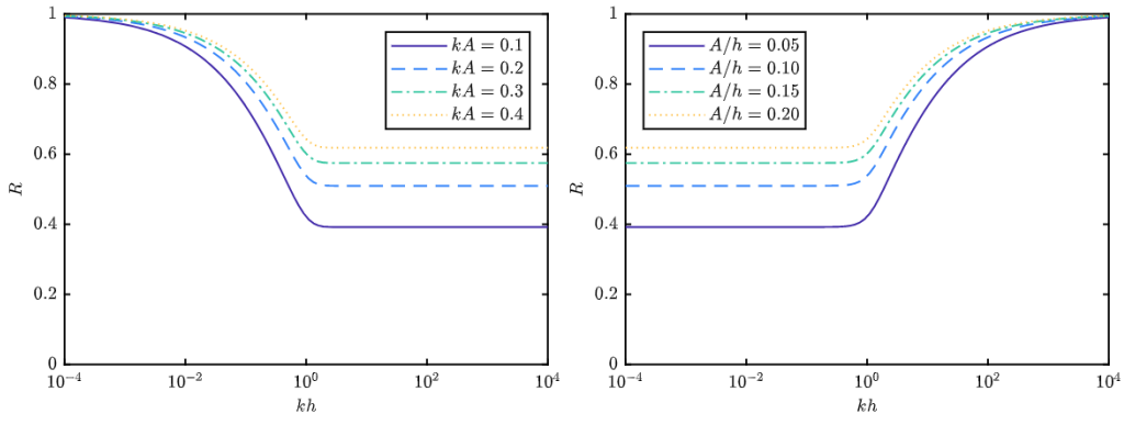
Fig. 8. Variation of R with kh for C_f = 100 and L = 0 , assuming constant steepness (left) and constant amplitude (right). Calculations made using method 1.
