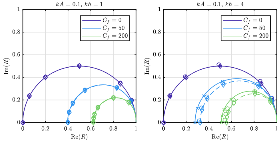
Fig. 16. Comparison of influence of inertia coefficient on R from analytic and BEM solutions. Solutions shown for C_f = 0, 50, 200 , kA = 0.1 , kh = 1 (left) and kh = 4 (right). Solid (dashed) lines represent solutions using method 1 (2) for 0 \leq kL < \infty . Circles represent BEM solution for kL = 0, 0.5, 1, 2, 5, 10 . Crosses (diamonds) represent analytic solutions from method 1 (2) at the same values of kL .
