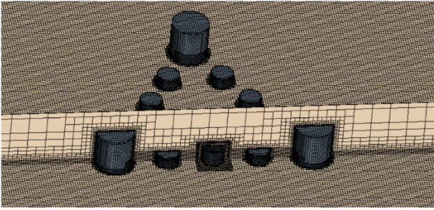
Fig. 13. Computation domain of the hybrid system for the free decay test.
