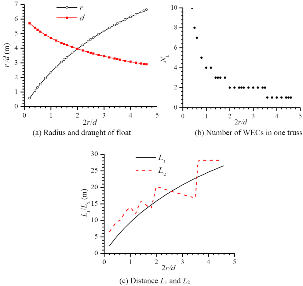
Fig. 6. The size and layout of initial selected WECs for T_p = 4.94 s.
