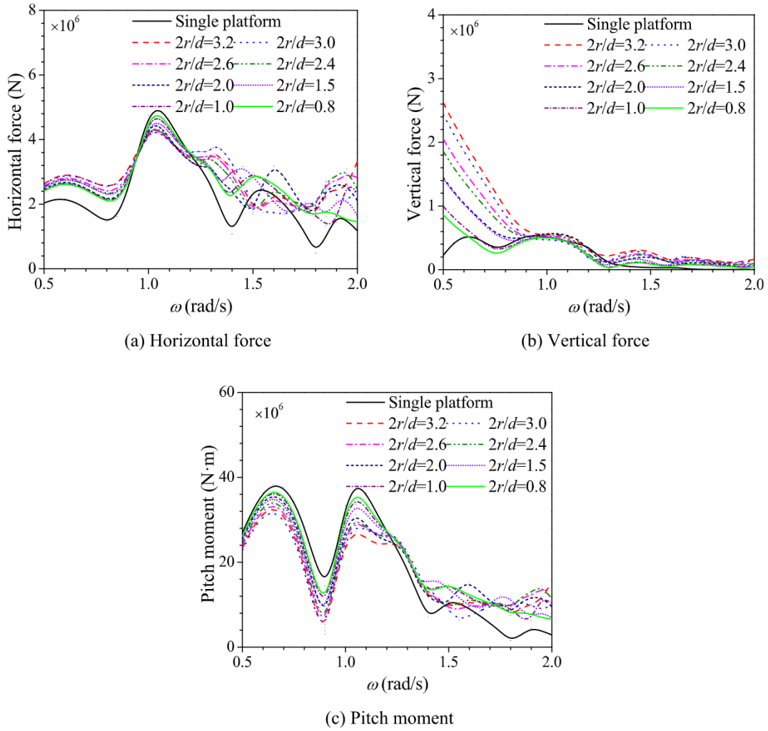
Fig. 20. Variations of horizontal force, vertical force, and pitch moment versus \omega with different 2r/d .
