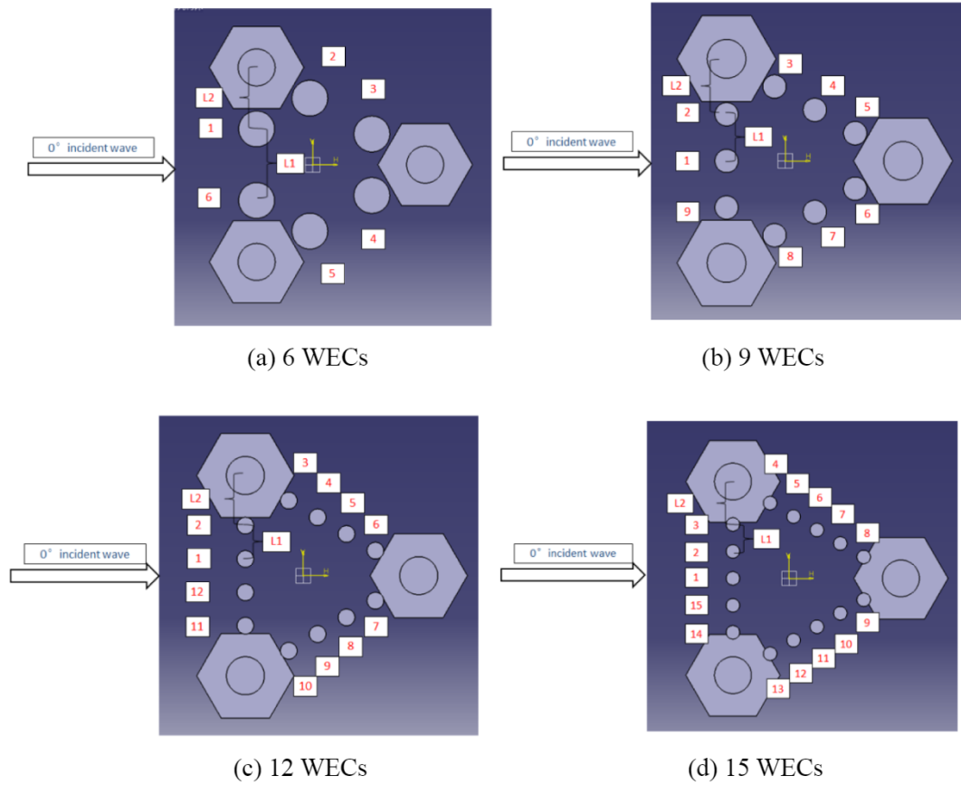
Fig. 7. Plan view of four different layouts of WECs.
