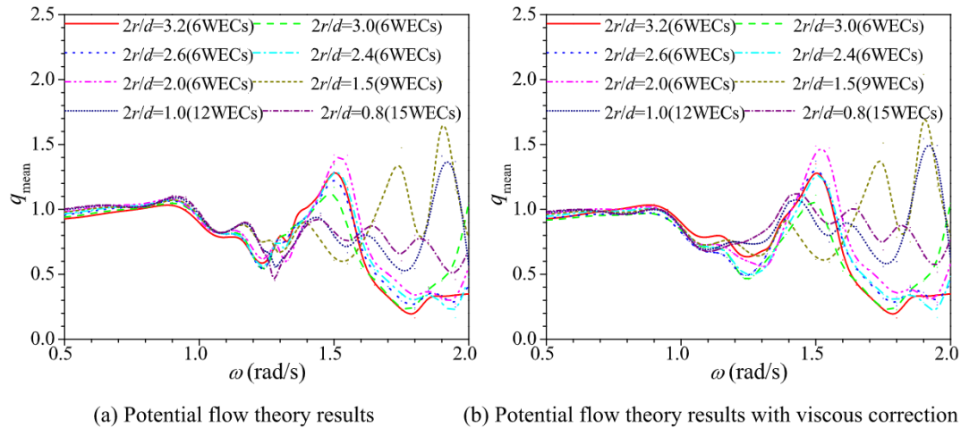
Fig. 19. Variations of mean interaction factor q_{mean} versus \omega with different 2r/d .
