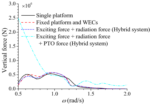
Fig. 21. Different components of vertical force for 2r/d = 3.2 .
