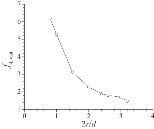
Fig. 15. Variation of non-dimensional viscous damping correction coefficient f_{A,visc} versus 2r/d .
