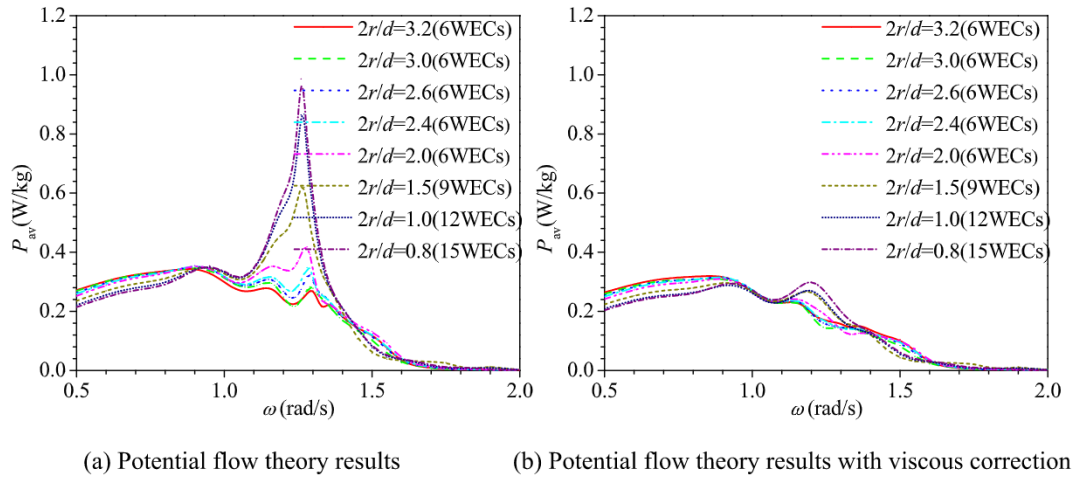
Fig. 17. Variations of total wave power per unit weight P_{av} versus \omega with different 2r/d .
