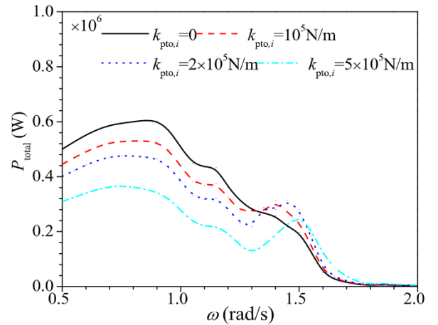
Fig. 22. Comparisons of wave power with different k_{pto,i} for 2r/d = 3.2 .
