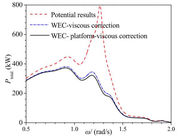
Fig. 14. Comparison of the total wave power vs. \omega between the uncorrected potential flow results, the potential results with viscous correction for a single WEC and the potential results with viscous correction for the hybrid system.
