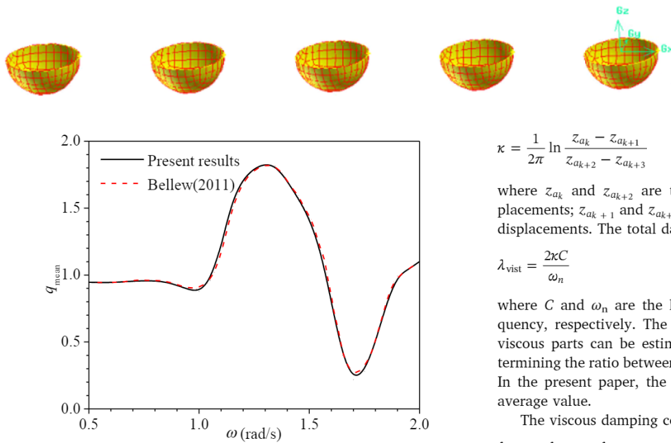
Fig. 4. Comparison of the mean interaction factor between the present results and the published numerical results in [40].
