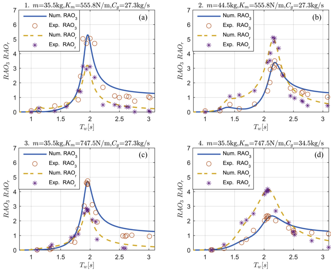
Fig. 20. Comparison of the motion responses (outer-floater motion and internal-mass relative motion RAOs) between numerical and experimental results for different cases 1 to 4 (a ~ d) which have same PTO parameter as in bench test (Fig. 14).
