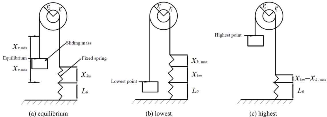
Fig. 3. The design sketch of the spring system and the three special positions of the sliding-mass during operation.
