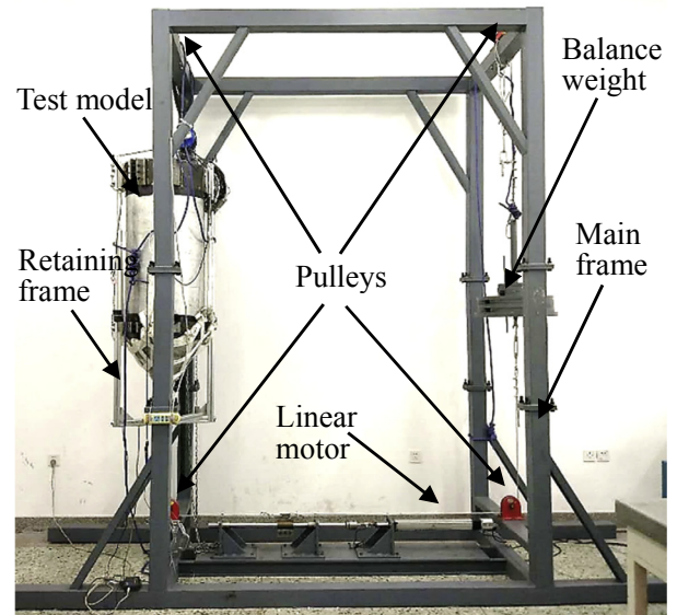
Fig. 11. The test bench with test model in position.
