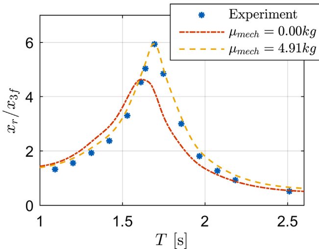
Fig. 8. The motion response comparison with and without the mechanical added mass when m = 35.5 kg, K_m = 555.8 N/m, C_g = 0.0 kg/s.
