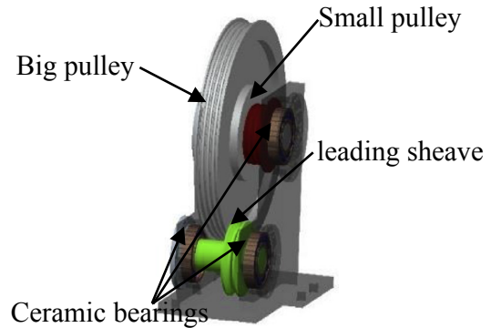
Fig. 4. The rendering of the stepped pulley.
