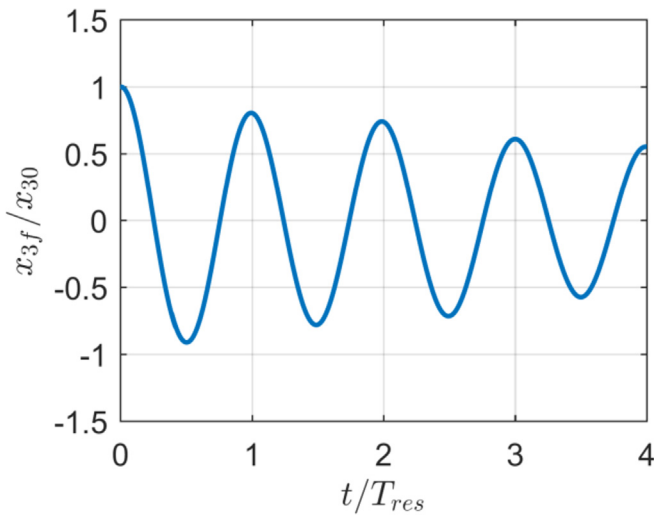
Fig. 17. Free decay curve of the outer-floater.
