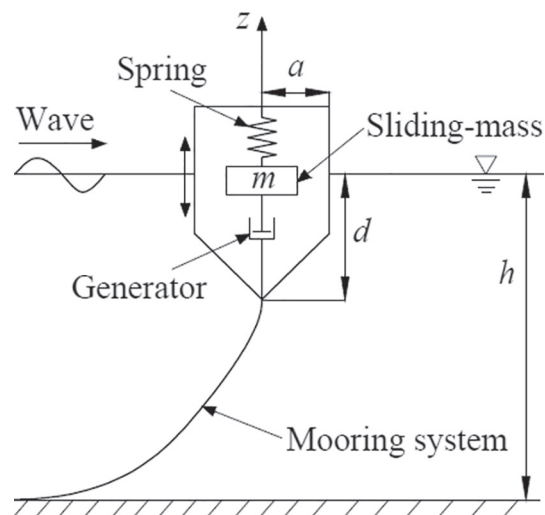
Fig. 1. The general schematics of the DR-WEC.
