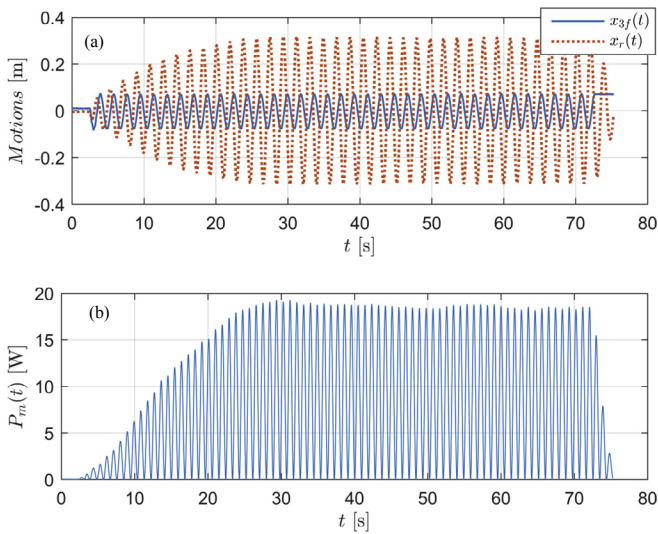
Fig. 13. Examples of the time histories of the motions (a) and power (b) when m = 44.5 kg, K_m = 555.8 N/m, C_g = 27.3 kg/s, and T = 1.8 s.
