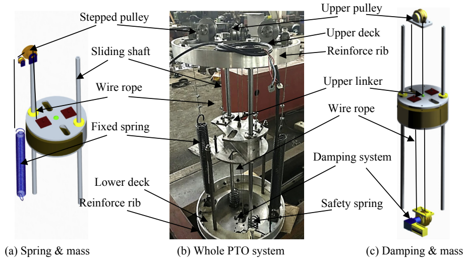
Fig. 7. The assembly of the BI-PTO system.
