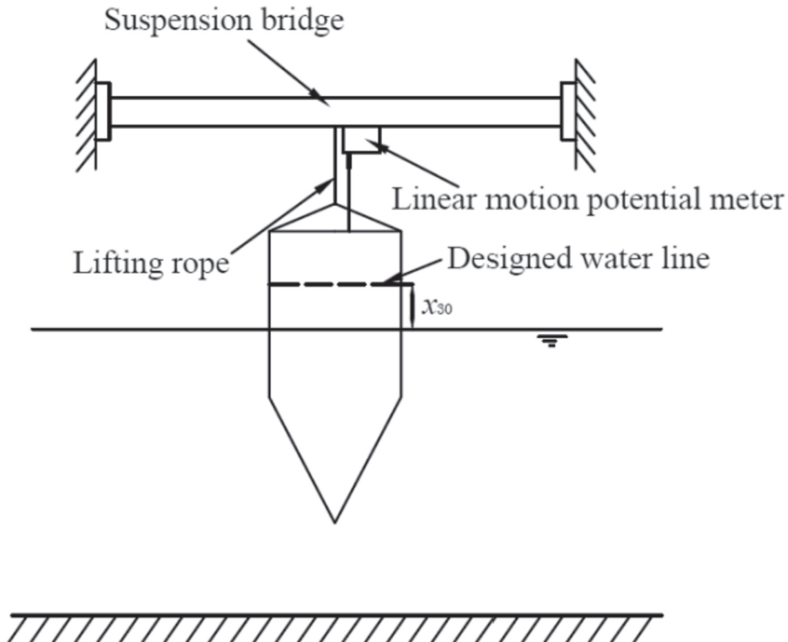
Fig. 16. Schematic of the free decay test.
