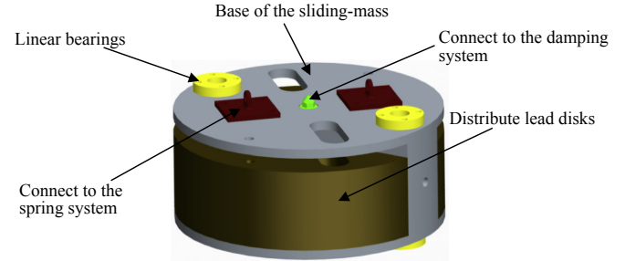
Fig. 5. The rendering of the sliding-mass.
