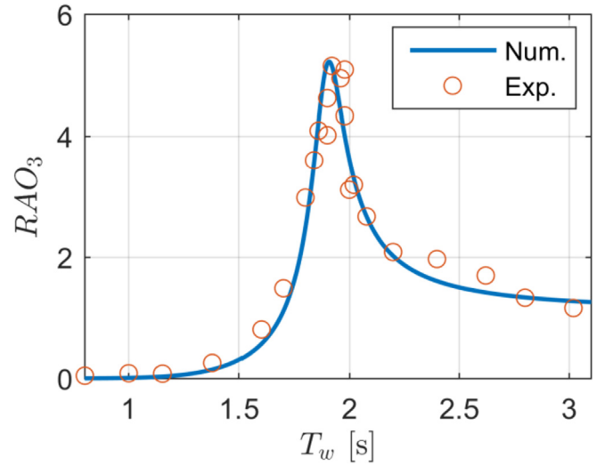
Fig. 19. Comparison of the outer-floater RAO between numerical and experimental results.
