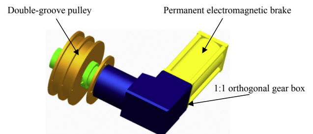
Fig. 6. The rendering of the damping system.
